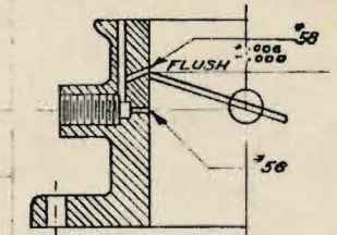
IDLE DISCHARGE HOLE LOCATION IN RELATION TO THE THROTTLE VALVE.
